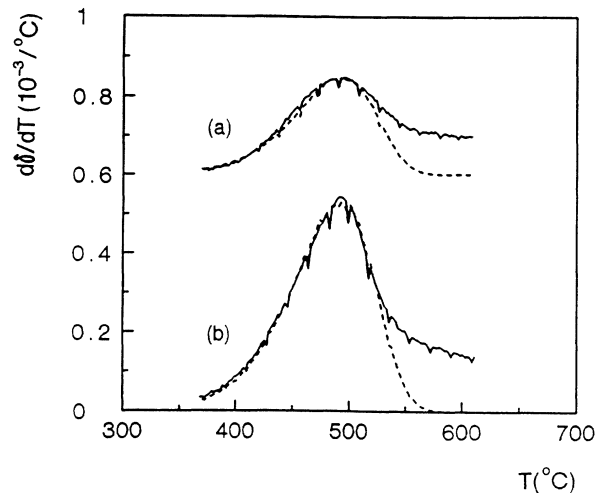
FIG. 5. Oxygen desorption curves of (a) (\text{Ca,Ba,Lu})\text{Cu}_3\text{O}_{7-\delta} ( \delta \approx 0.07 ) and (b) \text{YBa}_2\text{Cu}_3\text{O}_{7-\delta} ( \delta \approx 0.05 ), together with theoretical fits (dashed curves) for single-site desorption.
