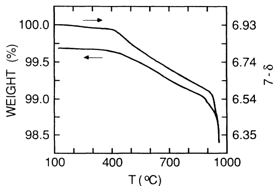
FIG. 4. Weight loss of (\text{Ca,Ba,Lu})\text{Cu}_3\text{O}_{6.93} measured thermogravimetrically at a heating and cooling rate of 7^\circ\text{C}/\text{min} in air. The right y axis shows the oxygen content of the sample calculated from the weight loss.
