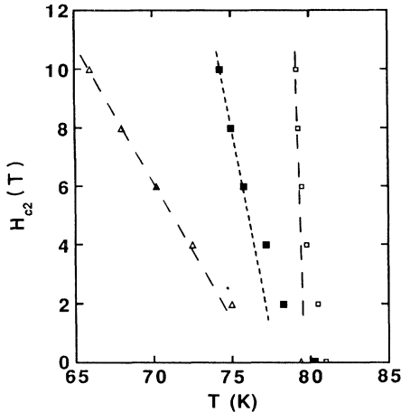
FIG. 3. Upper critical field H_{c2} vs temperature T curves for (\text{Ca,Ba,Lu})\text{Cu}_3\text{O}_{6.93} . Triangles, solid squares, and open squares indicate 10%, 50%, and 90% of the normal-state resistivity, respectively.
