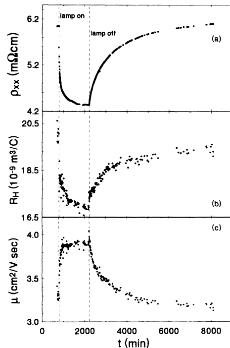
FIG. 2. Time dependence at room temperature during and after halogen white light illumination of the electrical resistivity \rho_{xx} , Hall coefficient R_H , and Hall mobility \mu = c(|R_H|/\rho_{xx}) , for an insulating \text{YBa}_2\text{Cu}_3\text{O}_{6.5} film.
