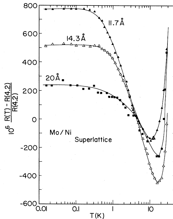
FIG. 2. Temperature dependence of normalized resistance for nonsuperconducting Mo/Ni structures. Again, the labels refer to \frac{1}{2}\Lambda .
