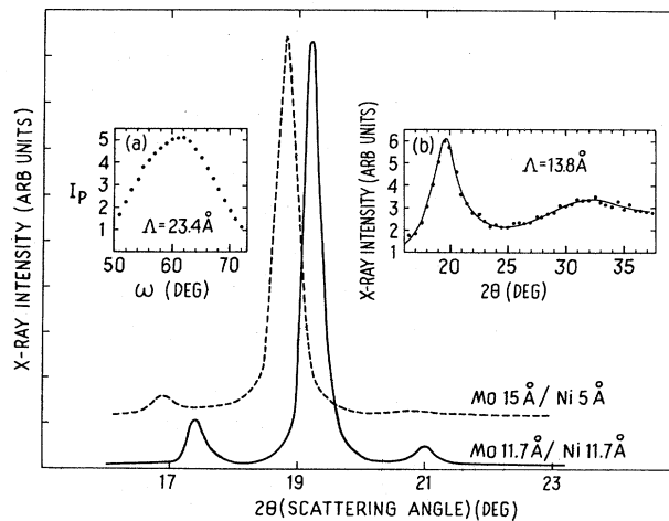
FIG. 3. 00/ x-ray diffraction profiles for two samples showing coherent satellites. Inset (a): Rocking curve for Mo 11.7 Å/Ni 11.7 Å. I_p is the intensity of the principal peak near 2\theta = 19^\circ . Inset (b): Glassy behavior of Mo 6.9 Å/Ni 6.9 Å sample.
