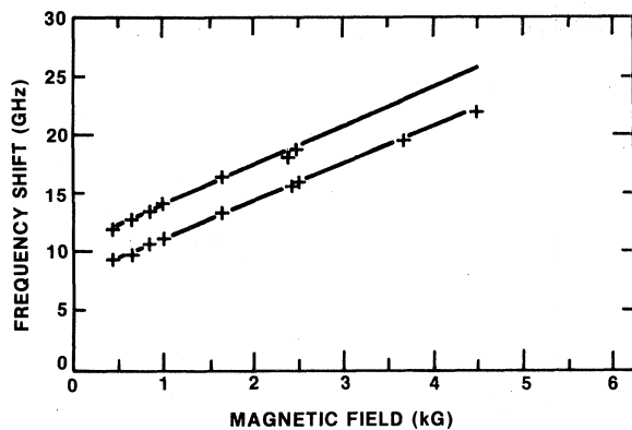
FIG. 6. Field dependence of the two modes observed in a superlattice with d_1=d_2=550 Å. The lines are fits according to Eqs. (1) and (5).
