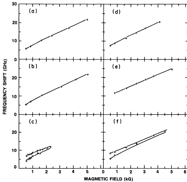
FIG. 4. Field dependence of magnon frequencies in a representative set of Mo/Ni superlattices. Solid lines are fits according to Eqs. (1) and (3). The samples are as follows: (a) d_1=100 Å, d_2=300 Å; (b) d_1=100 Å, d_2=100 Å; (c) d_1=138 Å, d_2=46 Å; (d) d_1=250 Å, d_2=750 Å; (e) d_1=5000 Å, d_2=5000 Å; and (f) d_1=540 Å, d_2=180 Å.
