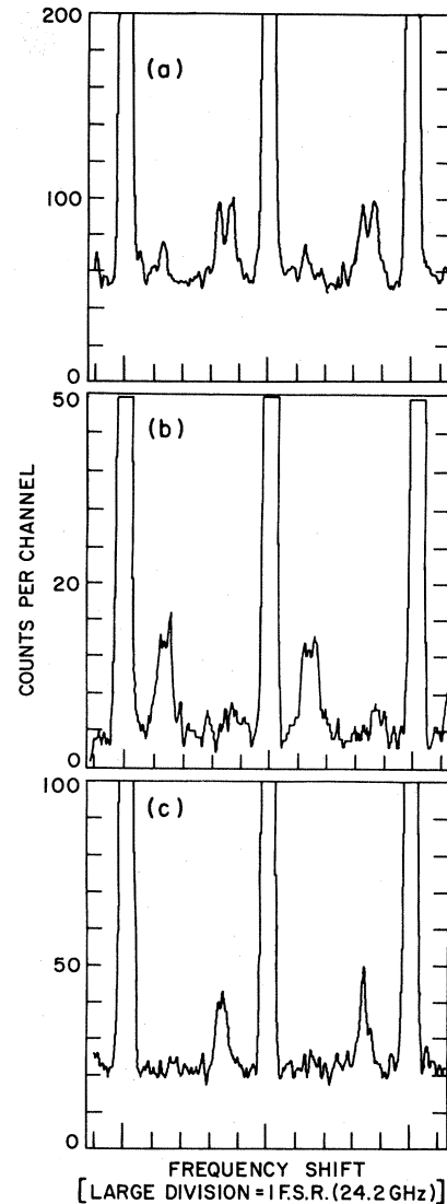
FIG. 3. Magnon spectra obtained from Mo/Ni superlattices with (a) d_1=3d_2=249 Å, applied field H=+0.93 kG; (b) d_1=d_2=160 , Å, H=-0.83 kG; and (c) 3d_1=d_2=300 Å, H=+0.93 kG. The direction of the frequency shift in (b) is different from that in (a) and (c) because the field direction was reversed.
