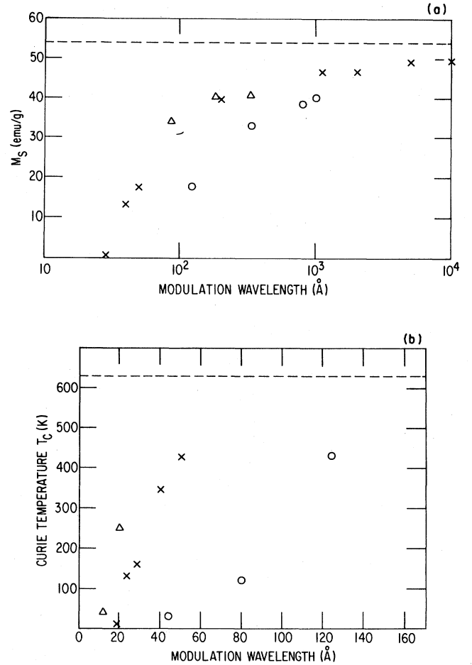
FIG. 1. (a) Magnetization and (b) Curie temperature for Mo/Ni superlattices. Triangles are for d_1 = 3d_2 , crosses are for d_1 = d_2 , and circles are for 3d_1 = d_2 . Dashed lines represent the values for bulk Ni.
