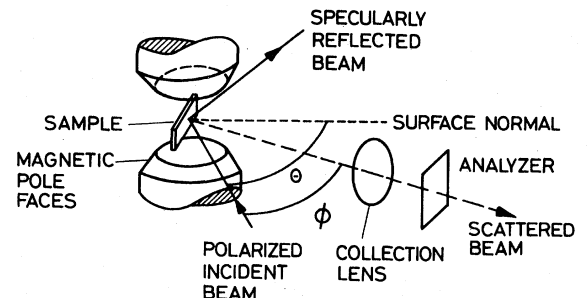
FIG. 2. Schematic diagram of the experimental arrangement used in our experiments.
