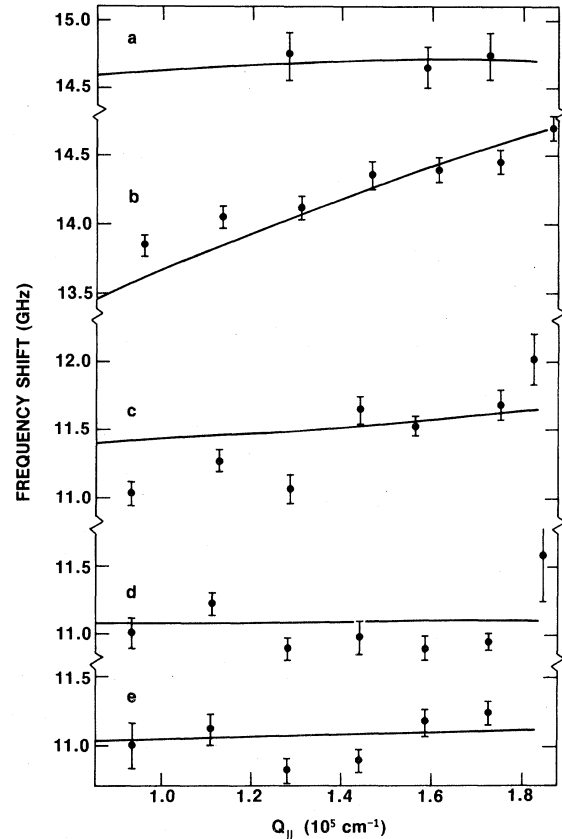
FIG. 5. Wave-vector dependence of magnons in a representative set of Mo/Ni superlattices. Solid lines are fits according to Eqs. (1) and (2). Magnetic field was 2.11 kG. The samples were as follows: a, d_1=d_2=2500 Å; b, d_1=d_2=550 Å; c, d_1=d_2=250 Å; d, d_1=d_2=100 Å; and e, d_1=249 Å, d_2=83 Å.
