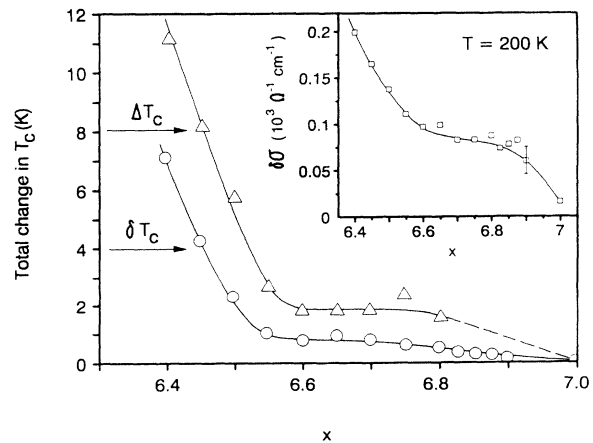
FIG. 3. Total enhancement of the critical temperature after the illumination \delta T_c as a function of the oxygen content. The data are compared to the total increase of T_c due to oxygen ordering effects \Delta T_c in YBCO single crystals (Ref. 13). The inset shows the total increase of the conductivity at T = 200 K after the illumination. All the solid lines are guides to the eye.
