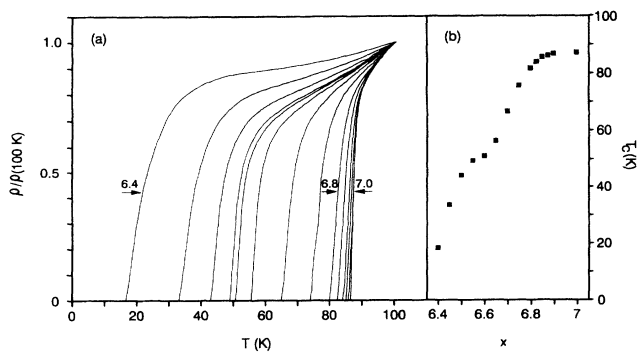
FIG. 1. (a) Normalized resistive transitions for a 1000-Å-thick YBCO film with different oxygen contents x . Between x = 6.4 and 6.8 the oxygen content has been varied in steps of 0.05, while between x = 6.8 and 6.9 the step is 0.025. (b) Critical temperature as a function of the oxygen content.
