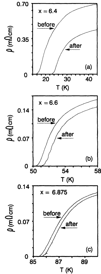
FIG. 2. Resistive transitions for the YBCO film of Fig. 1(a) before and after the laser illumination and for different oxygen contents x . Notice the parallel shift of the transitions towards higher temperatures after the illumination.
