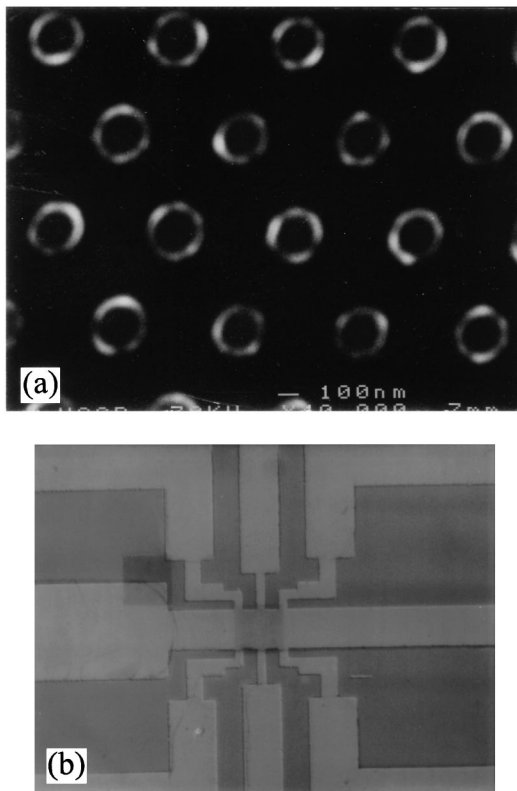
FIG. 1. (a) SEM image of a triangular array of Fe magnetic dots fabricated by e -beam lithography on a Si substrate. The lattice constant is d = 600 nm and the Fe dots have a radius r = 100 nm. (b) Micrograph of the Nb bridge defined by optical lithography in the array region. The width is 40 \mu\text{m} and the distance between the voltage contacts used for transport measurements is 50 \mu\text{m} .
