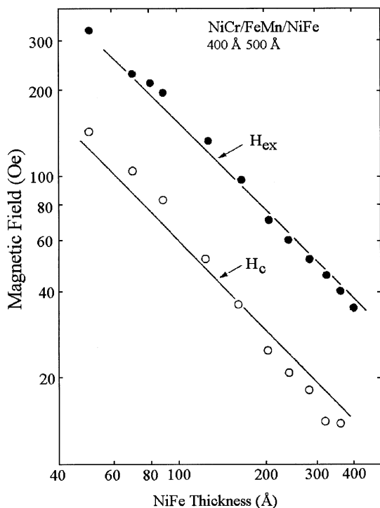
Fig. 9. Dependence of exchange bias H_E (filled symbols) and coercivity H_C (open symbols) with the FM layer thickness for \text{Fe}_{80}\text{Ni}_{20}/\text{FeMn} at a fixed t_{\text{AFM}} = 50 \text{ nm} [208].
