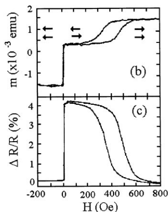
Fig. 4. (a) Schematic diagram of a spin valve device. (b) Hysteresis loop, m(H) , and (c) magnetoresistance, \Delta R/R(H) , of \text{Fe}_{20}\text{Ni}_{80}/\text{Cu}/\text{Fe}_{20}\text{Ni}_{80}/\text{FeMn} GMR spin valve at room temperature [23].
