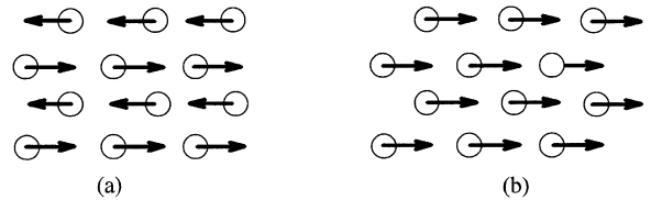
Fig. 7. Schematic spin diagram for a (a) compensated and (b) uncompensated AFM surface.
