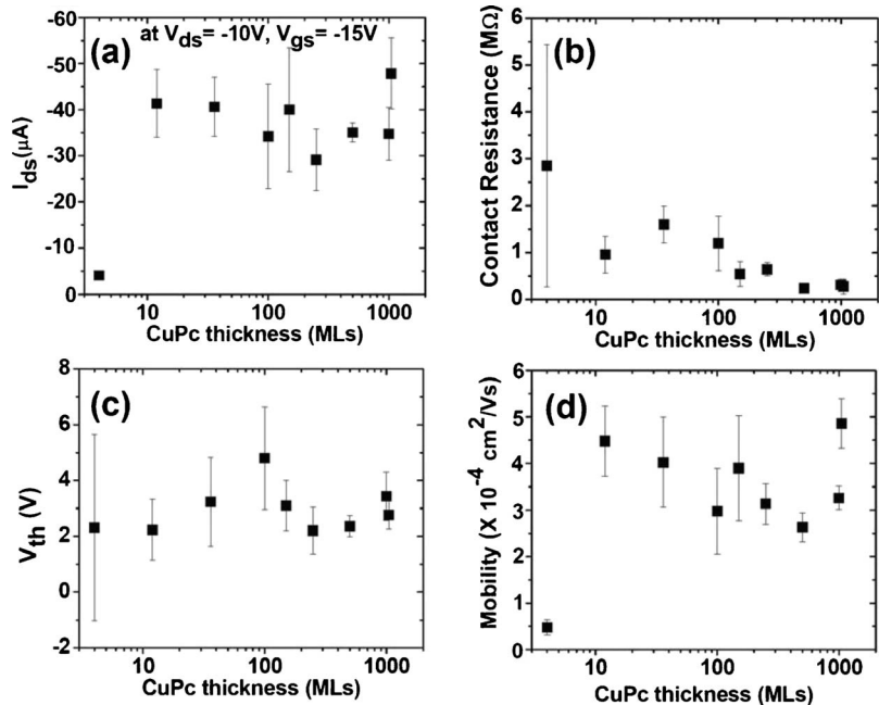
FIG. 7. (a) On-state current at V_{ds}=-10 V, V_{g}=-15 V, (b) contact resistance, (c) threshold voltage, and (d) mobility as a function channel thickness from CuPc OTFTs fabricated with the bilayer photoresist lift-off process.
