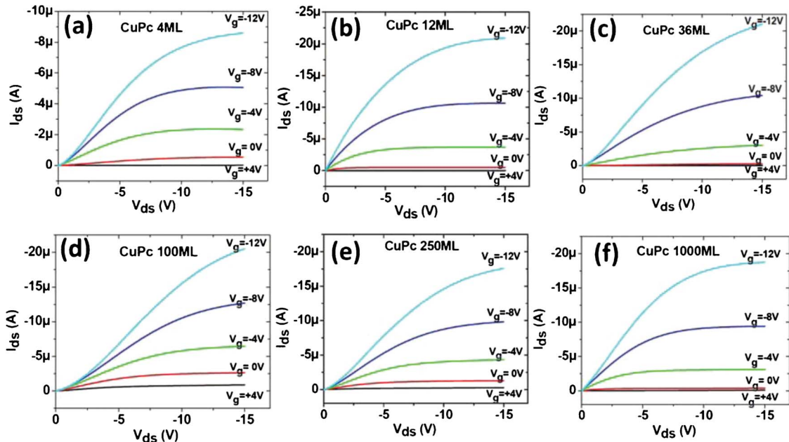
FIG. 5. (Color online) Representative output characteristics of CuPc OTFTs with different CuPc thicknesses. (a) 4, (b) 12, (c) 36, (d) 100, (e) 250, and (f) 1000 ML.
